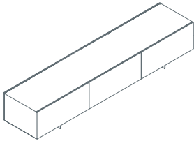
Cabinet with deep drawer lockable 1CE6041: L 200 D 65 H 54,5 1CE6042: L 298,5 D 65 H 54,5 1CE6043: L 200 D 65 H 54,5 (with finishing back) 1CE6044: L 298,5 D 65 H 54,5 (with finishing back)
